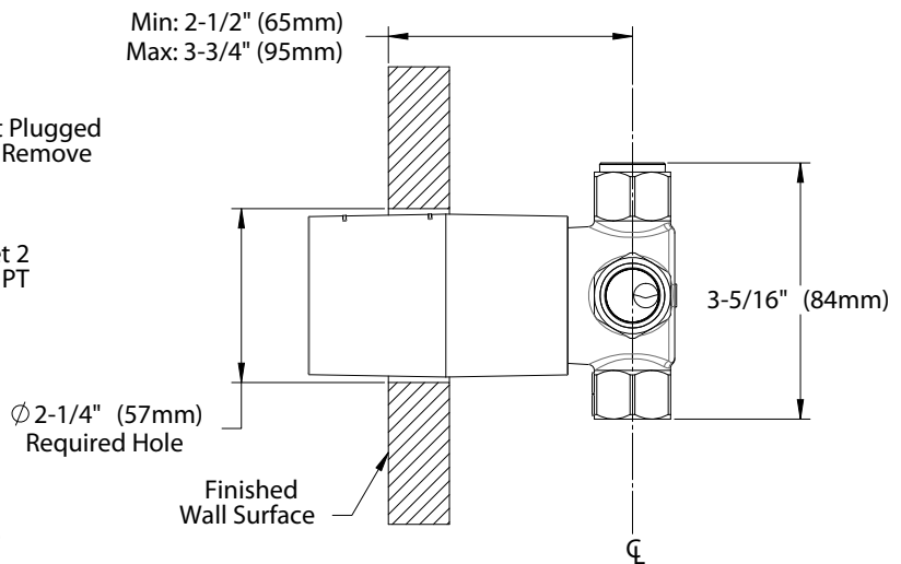
Valve shown with plaster guard in place
