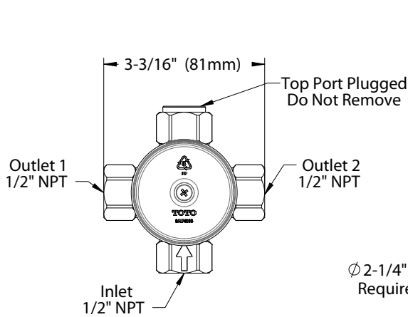
Valve shown with plaster guard in place
